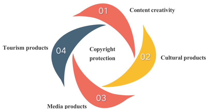
Figure 2. Copyright protection
